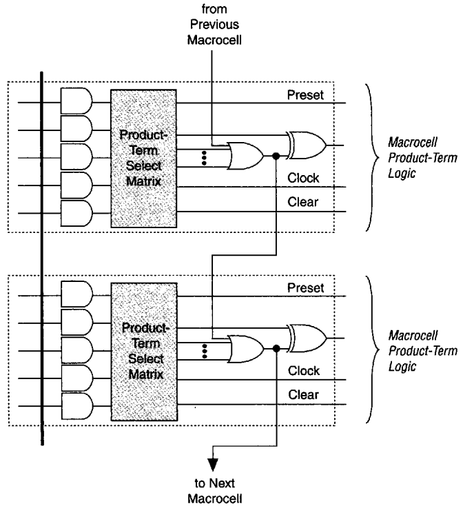
Figure 5. Parallel Expanders
